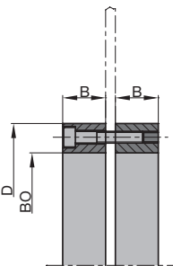
Set of spacers
