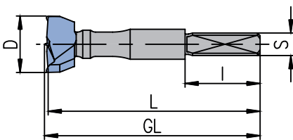
Z 2 / V 2 with centre point
