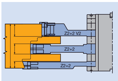
Application example ProFix C „frame tenon for top of jamba“: Cutting edges in RipTec design for improved quality of cut in cross grain. Combination of ProFix knives for large cutting widths in the rail area.
