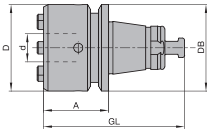
Collet chuck
