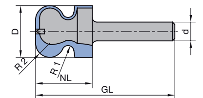
Finger pull cutter WO 532 1
