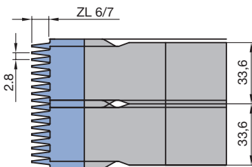
Minifinger joint cutter ZL 6/7 mm, TG 2.8 mm
