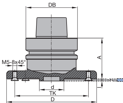
Clamping variant with concentrically mounted sawblade
