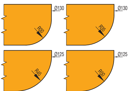
Profile cutterhead D-227 mm
