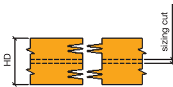
Profile 4 with shoulder cutters for splitting
